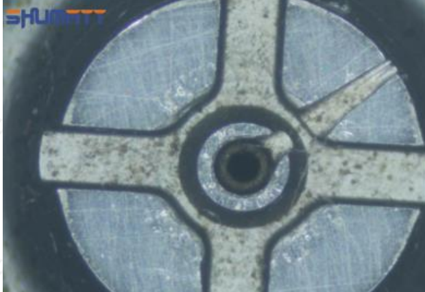
Washout marks caused by the presence of impurities in the fuel
